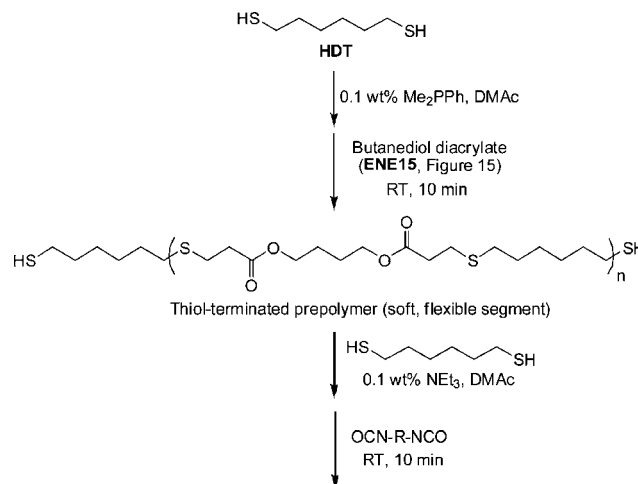
Scheme 27 Outline for the preparation of segmented polythiourethanes via sequential thiol-ene/thiol-isocyanate processes.
