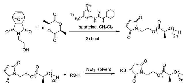
Scheme 23 The synthesis of α-functional thioether polyactides via ring-opening polymerization of lactide with a furan-protected maleimide alcohol initiator followed by a [4 + 2] cycloaddition and base-mediated thiol-ene coupling.
