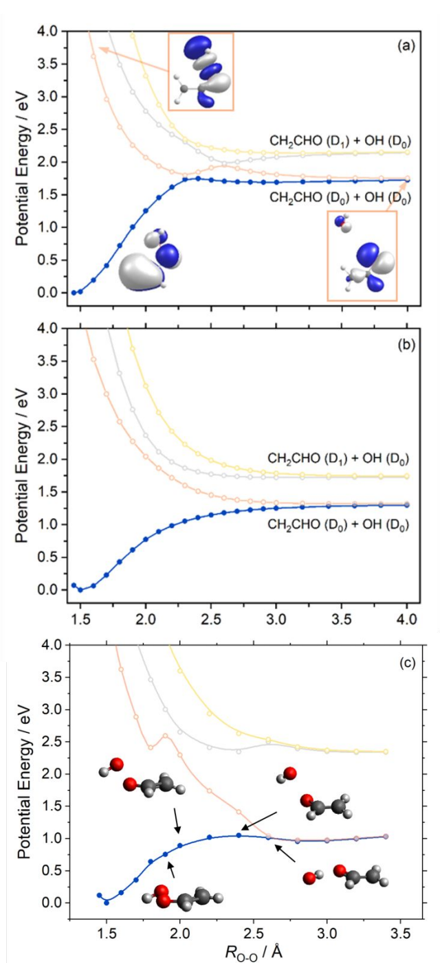
Figure 5: unrelaxed adiabatic PE profile of VHP along the O-O stretch coordinate at (a) \tau_{\text{CCOO}} = 0^\circ and (b) \tau_{\text{CCOO}} = 90^\circ , calculated at the XMS-CASPT2/aug-cc-pVTZ level of theory. (c) XMS-CASPT2/AVTZ//CASPT2/AVTZ relaxed PE profiles along the R_{\text{OO}} coordinate.
