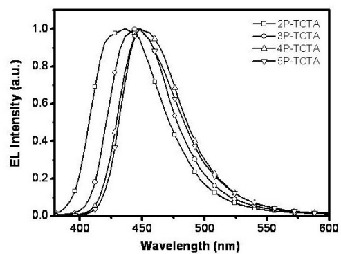
Figure 6. EL spectra for deep-blue emitters 2P-TCTA ~ 5P-TCTA at a driving voltage of 6 V.
