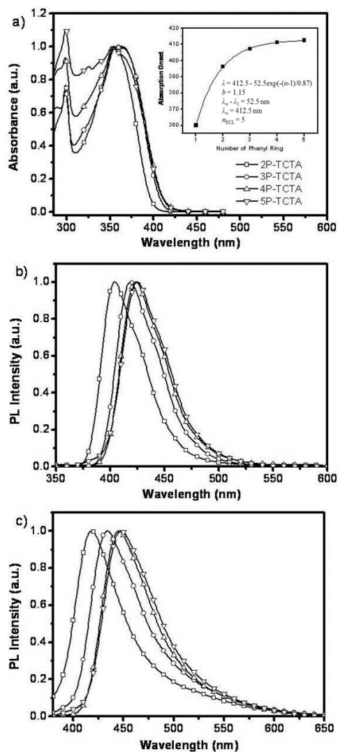
Figure 4. UV-Vis spectra in toluene (a), PL spectra in toluene (b), and PL spectra in solid states (c) for deep-blue emitters 2P-TCTA ~ 5P-TCTA. Inset: Correlation of the absorption onset and number of phenyl ring.
