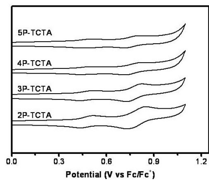
Figure 3. CV characteristics of deep-blue emitters 2P-TCTA ~ 5P-TCTA.
