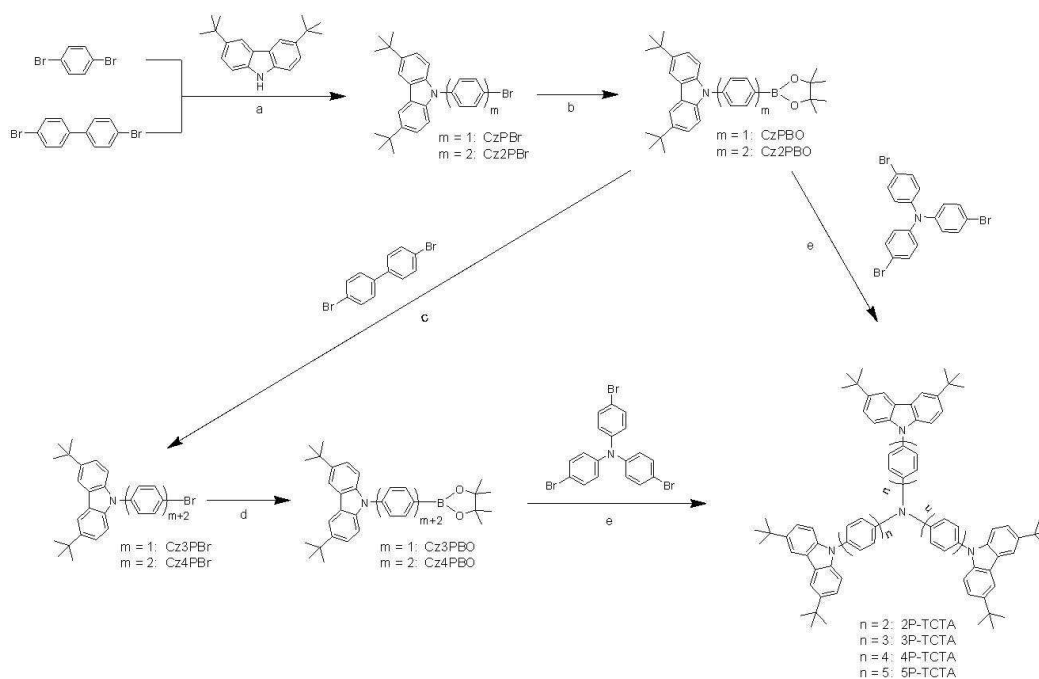
Scheme 1. Synthesis of TCTA-based deep-blue emitters.
