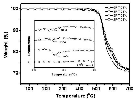
Figure 1. TGA curves of deep-blue emitters 2P-TCTA ~ 5P-TCTA and their DSC traces (inset).
