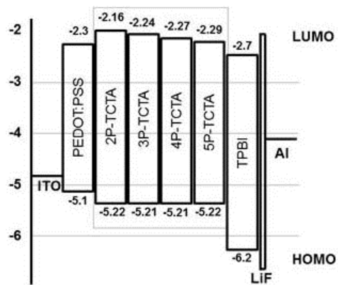
Figure 8. Energy level diagrams of devices based on 2P-TCTA ~ 5P-TCTA.
