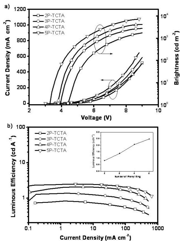
Figure 7. The current density—voltage—brightness characteristics, and the current density dependence of the luminous efficiency for deep-blue emitters 2P-TCTA ~ 5P-TCTA. Inset: the correlation of the luminous efficiency and number of phenyl ring.
