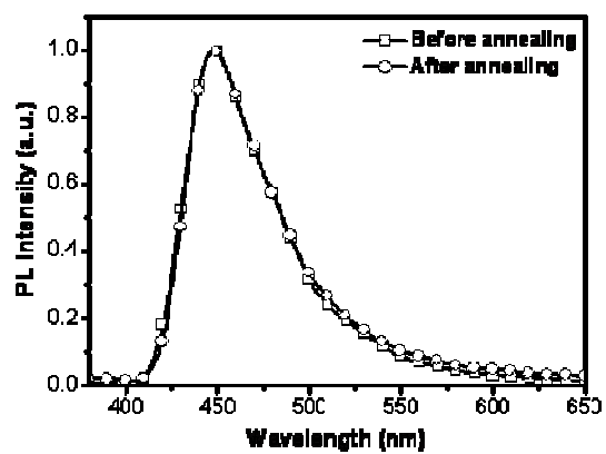
Figure 5. PL spectra of 5P-TCTA film before and after annealing at 150 °C for 2 hours in air.
