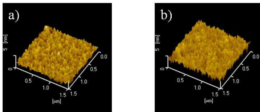
Figure 2. Comparison of AFM topographic images for 5P-TCTA between the pristine film (a) and annealed film (b).
