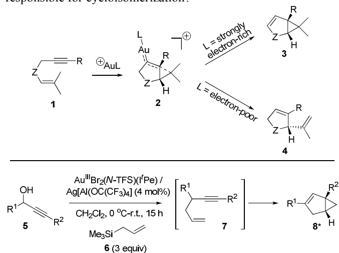
Scheme 1. Top: 1,5-enyne cycloisomerization showing how L can direct selectivity (3 & 4 representative products; others possible). Bottom: a tandem nucleophilic substitution-1,5-enyne cycloisomerization – thermal 1,3-rearrangements are possible for 8 (R 1 /R 2 = aryl groups).
