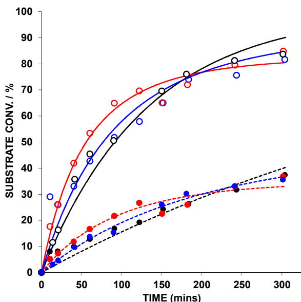
Figure 5. Kinetic profile for the concurrent cycloisomerisation of 4-phenyl-1-hexen-5-yne ( 9 ) and dimethyl allylpropargylmalonate ( 11 ) mediated by selected Au catalysts. Key: 1,5-enyne conversion ( 9 , open circles) and 1,6-enyne conversion ( 11 , closed circles) – black = AuBr(I'Pe); blue = AuBr 2 ( N -TFS)(I'Pe); red = AuBr 2 ( N -phthal)(I'Pe). Conditions: 0.2 M 9 , 0.2 M 11 in 1,2-dichloroethane, 1 mol% Au, 1 mol% AgOTf, 25 °C. 1, n -enyne ( n = 5 or 6) conversion monitored by GC analysis – each sample point was quenched by addition of ( n -Bu) 4 NBr. The kinetic curves were fitted using Dynafit™ with standard errors ~ 5%.
