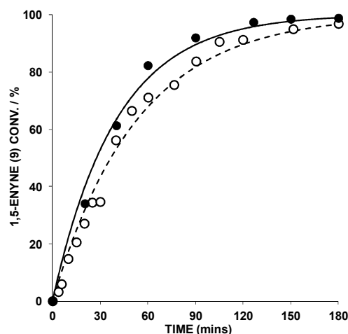
Figure 2. Effect of AgOTf equivalents relative to AuBr 2 ( N -TFS)(I'Pe) in 1,5-enyne cycloisomerisation of 9 (key: ● = 2 mol% AgOTf; ○ = 1 mol% AgOTf). Other details: [ 9 ] = 0.2 M, DCE, 1 mol% Au cat., 25 °C; 1,5-enyne conversion was monitored by HRGC – each sample point was quenched by addition of N ( n -Bu) 4 Br. The kinetic curves were fitted using Dynafit™.
