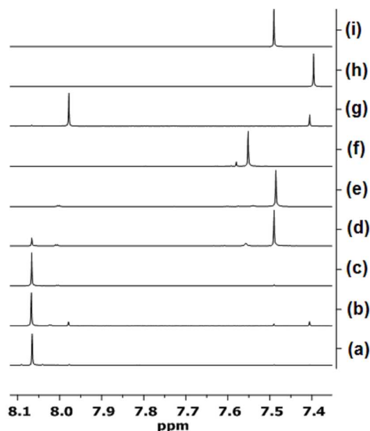
Figure 7. 1 H NMR spectroscopic analysis of the reaction of AuBr 2 ( N -TFS)(I'Pe) with AgOTf in acetone- d 6 over time. (a) AuBr 2 ( N -TFS)(I'Pe) only; (b) AuBr 2 ( N -TFS)(I'Pe), aged for 48 h; (c) AuBr 2 ( N -TFS)(I'Pe)/AgOTf (1:1), 10 mins; (d) as for (c), 4.5 h; (e) as for (c), 22.5 h; (f) AuBr(I'Pe)/AgOTf (1:1), 22.5 h; (g) solution of AuBr 3 (I'Pe) only, aged for 48 h; (h) AuBr(I'Pe) only; (i) Au( N -TFS)(I'Pe) only.
