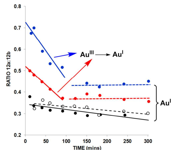
Figure 6. Product distribution from the cycloisomerization of 11 → 12a and 12b over time (data extracted from the kinetic profiles given in Figure 5 – closed black circles = AuBr(I'Pe); open black circles = AuBr(I'Pe) / 1,6-enyne 11 only; closed blue circles = AuBr 2 ( N -TFS)(I'Pe); closed red circles = AuBr 2 ( N -phthal)(I'Pe). The trendlines added to the graph serve as a guide to the eye.
