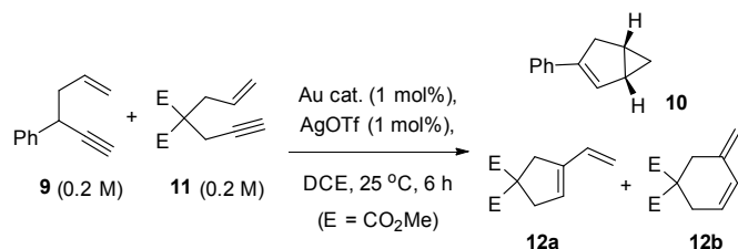
Scheme 3. Competition experiment of a 1,5-enyne 9 and 1,6-enyne 11 . Product 11 derives from 9 and products 12a and 12b from 11 . The kinetic profiles are shown in Figure 6 and product distributions of 12a:12b shown in Figure 7.
