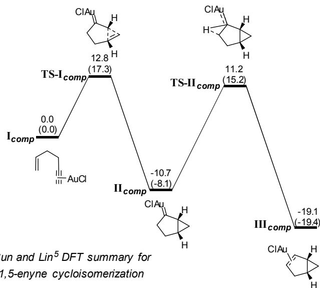
Scheme 4. Top: proposed mechanism for the 1,5-enyne cycloisomerization 9 → 10 (a role for Ag is not shown in the mechanism, although this cannot be ruled out). Bottom: DFT computed energies for the intermediates and transition states for the a 1,5-enyne cycloisomerization mediated by AuCl, reported by Sun and Lin.
