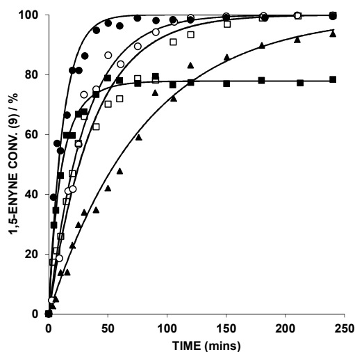
Figure 3. Effect of 1,5-enyne concentration [ 9 ] on the kinetics in a reaction mediated by various Au catalysts (1 mol%), AgOTf (1 mol%), in DCE at 25 °C (key: closed circles = AuBr(I'Pe); open circles = AuBr 2 (N-TFS)(I'Pe); closed squares = AuBr 3 (I'Pe); open squares = AuBr 2 (N-phthal)(I'Pe); closed triangles = AuBr 2 (N-phthal)(IMes)). 1,5-Enyne conversion monitored by HRGC analysis – each sample point was quenched by addition of ( n -Bu) 4 NBr. The kinetic curves were fitted using Dynafit™ with standard errors < 5%.
