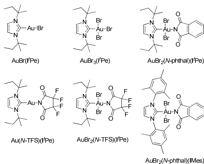
Figure 1. The structures of the catalysts used in this mechanistic study.
