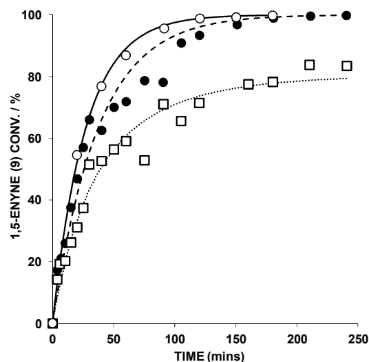
Figure 4. Effect of 1,5-enyne concentration [ 9 ] in a reaction mediated by AuBr 2 (N-phthal)(I'Pe) (1 mol%), AgOTf (1 mol%), in DCE at 25 °C (key: ○ = 0.1 M 9 ; ● = 0.2 M 9 ; □ = 0.5 M 9 ). 1,5-Enyne conversion monitored by GC analysis – each sample point was quenched by addition of ( n -Bu) 4 NBr. The kinetic curves were fitted using Dynafit™.
