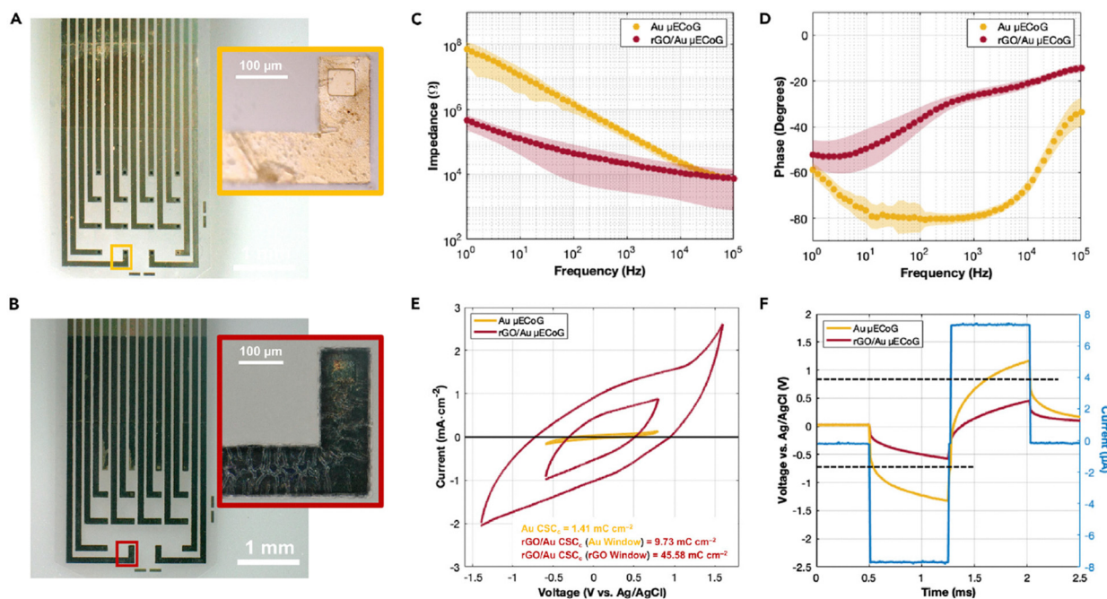
Fig. 9 Optical microscopy images of (A) bare Au and (B) rGO-coated microelectrodes with 50 × 50 μm contact openings. EIS (C) and (D), CV (E) and voltage transient measurements (F) of bare Au and rGO-coated electrodes. Reproduced from ref. 44 with permission from Elsevier, Copyright 2022.
