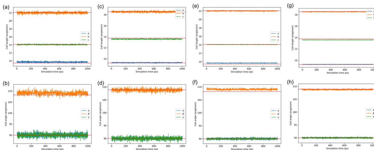
Fig. 4 Unit cell parameters obtained from 1 ns NPT simulation trajectories using a 2 \times 1 \times 2 supercell for tIIIm- \alpha (a) and (b) and tIIIm- \beta (c) and (d). Unit cell parameter of 1 ns NPT simulation trajectory using a 4 \times 3 \times 3 supercell for tIIIm- \alpha (e) and (f) and tIIIm- \beta (g) and (h). The red dash lines in the figure represent the lattice parameters of the experimental structures. All the parameters shown in the figure have been converted to the primitive cell parameters for better comparison with experimental data.
