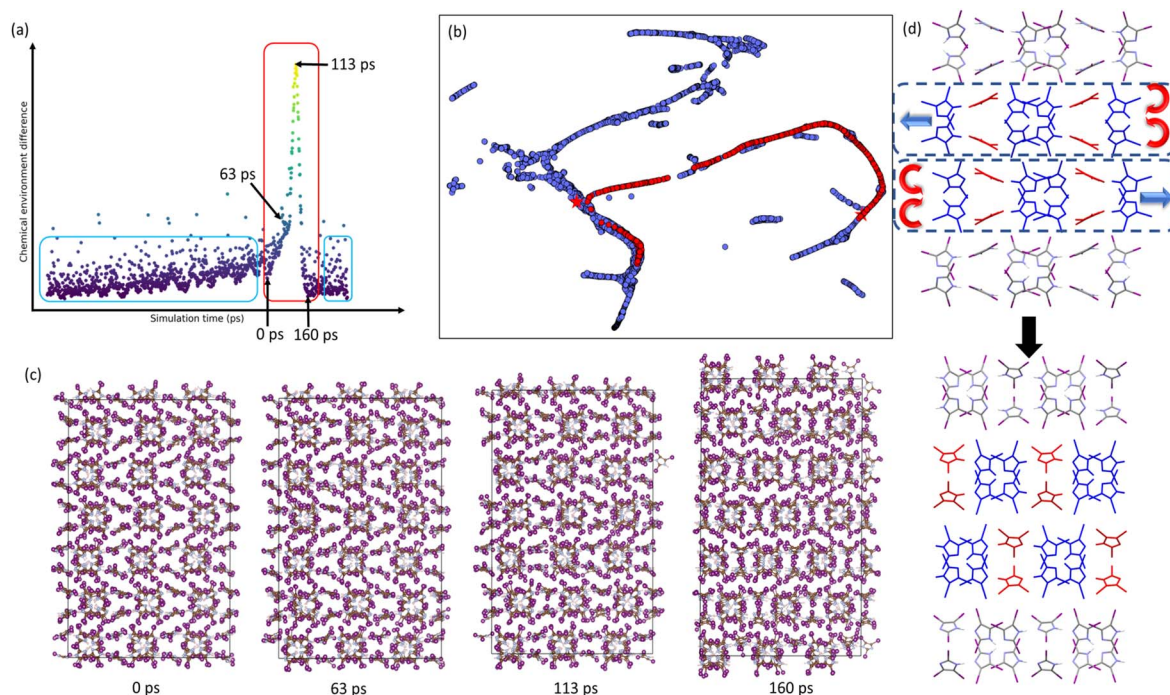
Fig. 6 (a) The chemical environment difference as a function of simulation time during the simulation starting from structure tIIIm- \beta following transformed to tIIIm- \alpha during reducing the pressure. The chemical environment difference is defined to measure the dissimilarity of one structure trajectory snapshot with other time-close snapshots based on SOAP descriptor. (b) 2D UMAP embedding of the SOAP space showing all the reference data (blue dots) and transformation process (red dots). Experimental structures are indicated by stars. (c) Snapshots from MD simulations depicting the phase transformation from tIIIm- \beta to tIIIm- \alpha . (d) A schematic diagram of the transition process from the tIIIm- \beta to the tIIIm- \alpha , where the molecules in red undergoing rotation and blue arrows indicating the slip direction of the entire layer.
