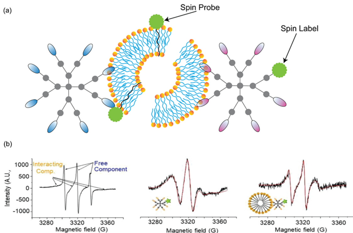
Fig. 9 Using EPR to study the interactions of a metallo dendrimers with liposomes. (a) Schematic of using the spin label (TEMPO) covalently attached to the dendrimer while the spin probe (4-( N,N -dimethyl N -dodecyl) ammonium-2,2,6,6-tetramethylpiperidine-1-oxyl bromide (CAT12)) was embedded with model membranes. (b) EPR spectra of the labelled dendrimers in the absence and presence of the model membranes. Left: an experimental EPR spectrum of dendrimers containing Ru(II) complexes in phosphate-buffered saline is shown as a representative example. Arrows indicate the presence of both free and interacting components. Middle and right: the experimental and simulated spectra corresponding to the interacting components of the dendrimers with Ru(II) complexes, either alone or in the presence of cetyltrimethylammonium bromide micelles. Adapted with permission from ref. 164. Licensed under a Creative Commons Attribution (CC BY) License.
