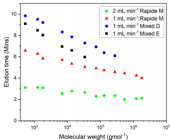
Fig. 3 Overlaid calibration samples using a Rapide M at 1 and 2 mL min and Agilent mixed E and D columns at a pumping speed = 1 mL min -1 .
