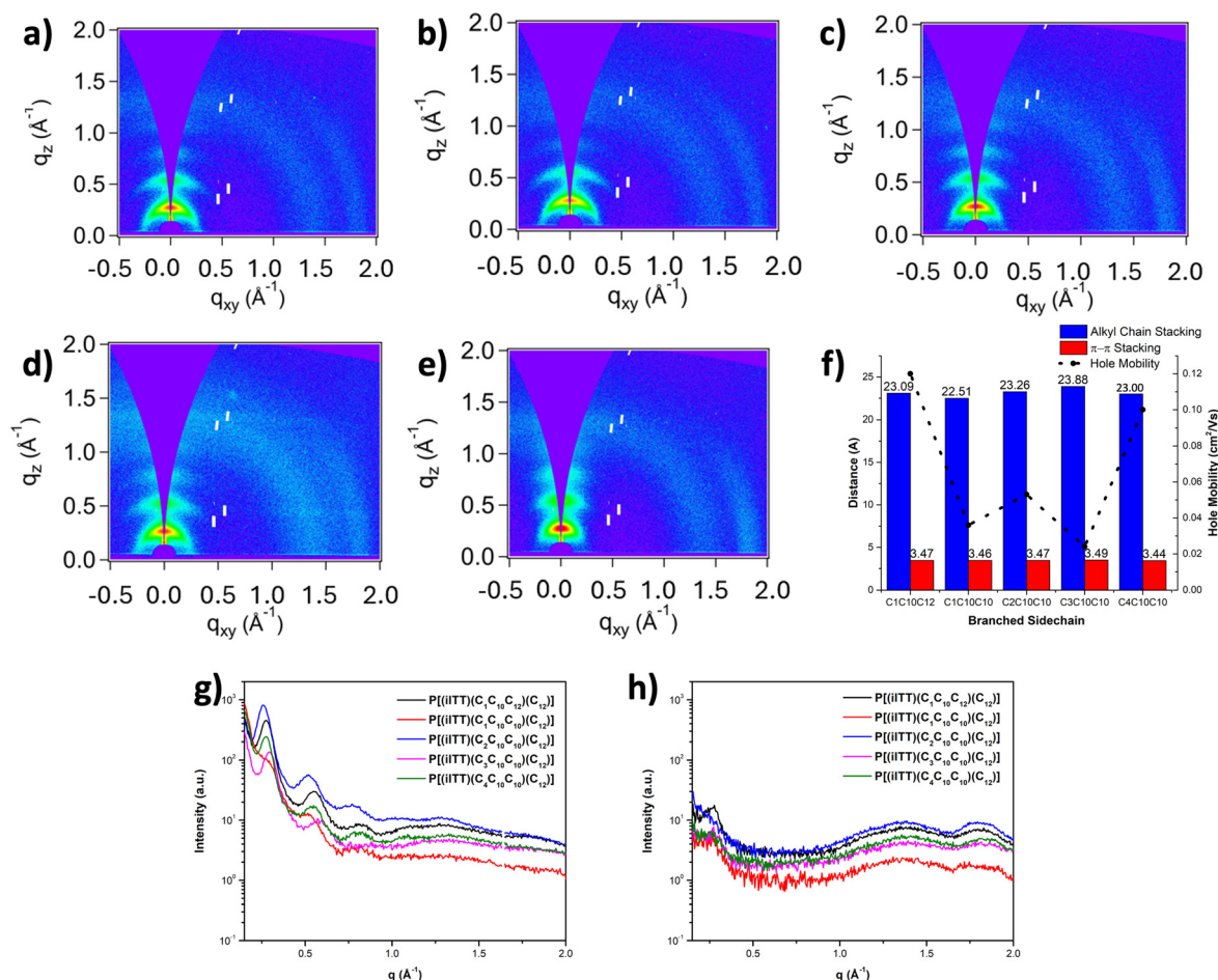
Fig. 3 Grazing incident wide-angle X-ray scattering (GIWAXS) 2D patterns of (a) P [(iTT)(C 1 C 10 C 12 )(C 12 )]]; (b) P [(iTT)(C 1 C 10 C 10 )(C 12 )]]; (c) P [(iTT)(C 2 C 10 C 10 )(C 12 )]]; (d) P [(iTT)(C 3 C 10 C 10 )(C 12 )]], and (e) P [(iTT)(C 4 C 10 C 10 )(C 12 )]]; (f) summary of chain distances (alkyl packing distance and \pi - \pi stacking) and hole mobility versus branching point; (g) out-of-plane and (h) in-plane 1D GIWAXS patterns. All measurements have been performed on thin films prepared from chlorobenzene solutions (10 mg mL −1 ) after thermal annealing at 150 °C.
