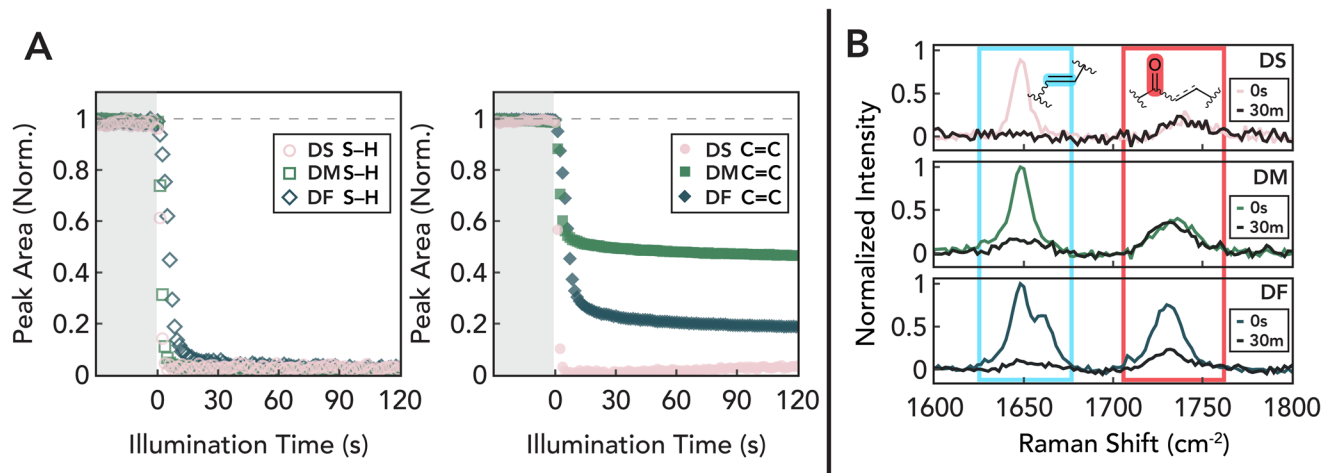
Fig. 6 (A) RT-FTIR-normalized peak area of thiol (left) and ene groups (right) in the photoreaction of DS, DM, and DF with HDT and 5% TATO. The thiol peak is quickly and quantitatively consumed along with the allyl peak of DS. However, the remaining peaks in DM and DF are associated with an overlapping internal ene of differing absorptions. (B) Raman spectroscopy shows conversion of ene groups and conversion of internal ene groups by the decrease in carbonyl peak intensity with the reduction in unsaturated conjugation.
