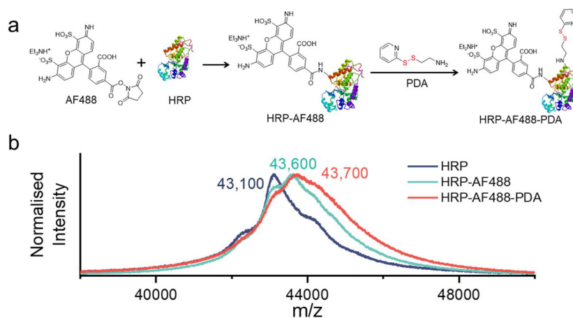
Fig. 3 (a) Reaction scheme of the modification of HRP with the fluorescent dye AF488 and disulphide bonds (PDA). (b) MALDI-TOF MS spectra in the [M + X]^+ ( X: \text{Na or H} ) range of HRP, HRP-AF488, and HRP-AF488-PDA.
