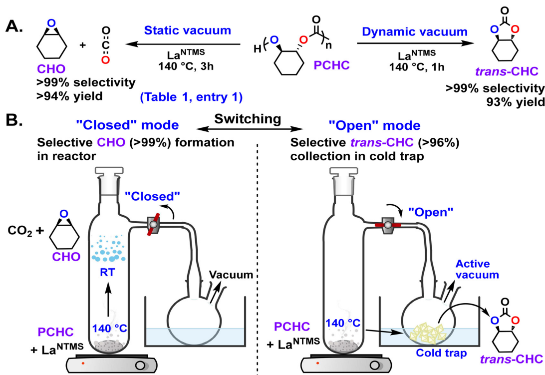
Fig. 2 A. Chemodivergent effects of reactor configuration on monomer selectivity in PCHC depolymerization. B. Reactor configured in switchable "Open" and "Closed" modes to yield their respective chemodivergent monomers in high yield and selectivity.
