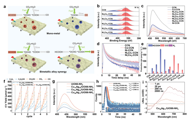
Fig. 5 (a) Schematic diagram of the reaction mechanism of photoreduction of CO 2 by the Ni x Cy-CCN catalyst. (b) XPS spectra of N 1s, (c) PL spectra and (d) time-resolved transient PL decay spectra for Ni x Cy-CCN. (e) Product evolution rates of Ni x Cy-CCN. Reproduced with permission from ref. 50. Copyright 2024, Wiley-VCH. (f) The cycling test over CuAg 50-x /UiO66-NH 2 . (g) PL spectra; (h) time-resolved transient PL decay spectra and (i) Fs-TA spectra of CuAg 50-x /UiO66-NH 2 . Reproduced with permission from ref. 51. Copyright 2024, Royal Society of Chemistry.
