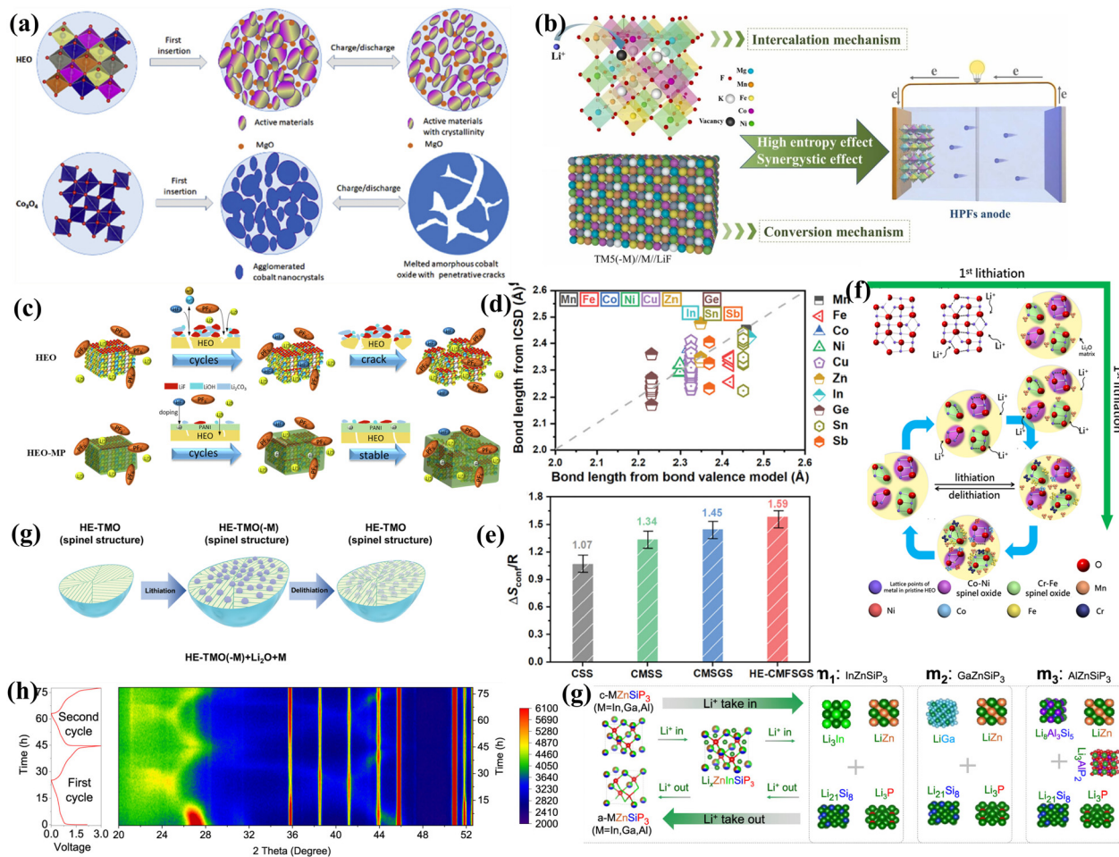
Fig. 12 (a) Schematic of cycling mechanisms of HEO and \text{Co}_3\text{O}_4 materials used as anodes for LIBs. 77 (b) High-entropy effect and synergistic effect of HEPFs. 192 (c) PANI interface on the HEO surface facilitates the inhibition of side reactions. 81 (d) Bond length calculated from bond valence model. (e) Calculated configurational entropy for different compositions. 43 (f) Schematic of the evolution of the atomic-scale microstructure of HEO during the cycling process. 181 (g) Illustration of lithiation/delithiation mechanism with the conversion reaction of HE-TMOs as anode of LIBs. 181 (h) Lithium storage mechanism of In (or Ga or Al) \text{ZnSiP}_3 silicon-based compounds. (i) Schematic of the generalized reaction mechanism of In (or Ga or Al) \text{ZnSiP}_3 . 183
