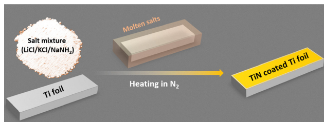
Scheme 1 Illustration of Ti surface nitriding process in molten salts.
