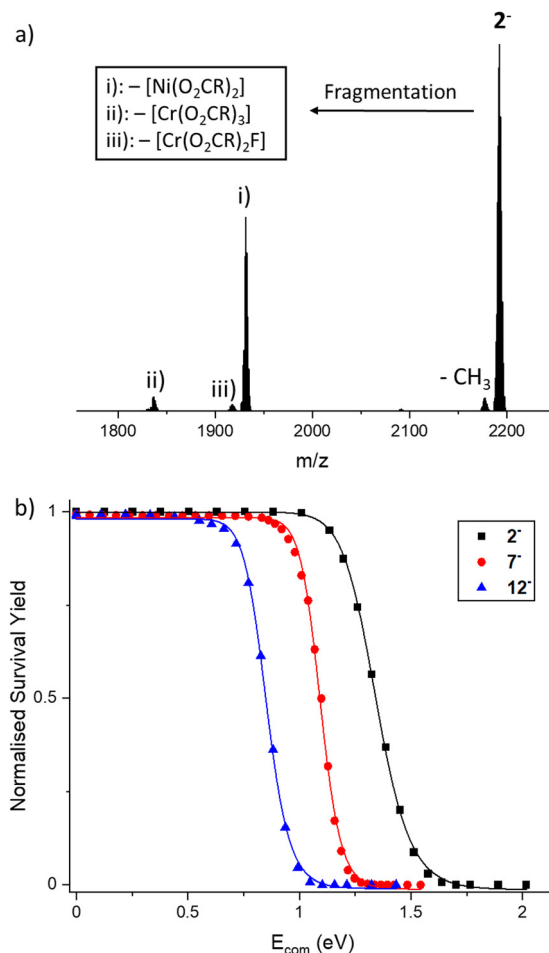
Fig. 3 (a) CID-MS spectrum of 2^- ( m/z = 2192 ) at E_{lab} = 105 eV. Besides the metastable loss of a methyl group from the carboxylate ligands, the three fragments (i), (ii) and (iii) were found that correspond to the losses of [Ni(O_2CR)_2] , [Cr(O_2CR)_3] and [Cr(O_2CR)_2F] , respectively. (b) Normalized survival yield vs. E_{com} fitted to a sigmoidal Hill function, exemplary for 2^- , 7^- and 12^- . The three ions follow the stability (and E_{50} value) order of 2^- > 7^- > 12^- (Fig. 2).
