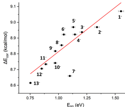
Fig. 4 Plot of the enthalpic contributions, \Delta E_{cor} , to the proton affinity computed for RCO_2^-/RCO_2H vs. E_{50} values. R^2 = 0.86 when excluding the outlier 7^- .
