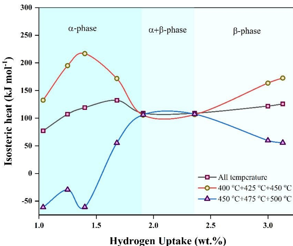
Fig. 5 Isosteric heat of hydrogen absorption ( Q_{st} ) as a function of hydrogen uptake for LiH-PSiNW alloy at different temperature zones
