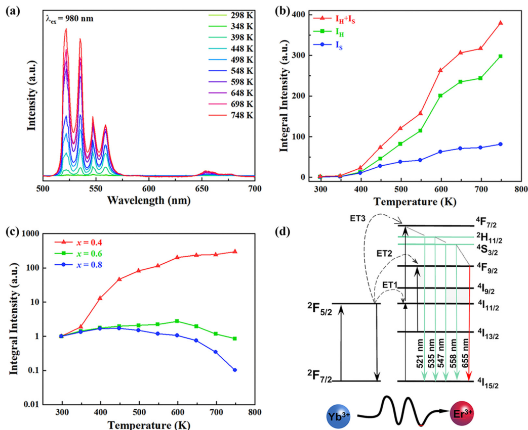
Fig. 6 (a) UCL emission spectra of the KM4 sample at 298–748 K under 980 nm laser excitation. (b) The corresponding UCL emission integral intensities of ^2H_{11/2(2)}/^2H_{11/2(1)} , ^4S_{3/2(2)}/^4S_{3/2(1)} and total ( ^2H_{11/2} + ^4S_{3/2} ) levels of Er^{3+} ions. (c) Integral intensity of KM4, KM6, and KM8 samples as a function of temperature. (d) Simplified energy level diagram to describe the ET process in the KM4 sample.
