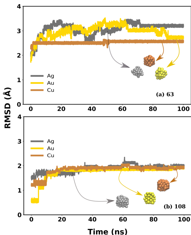
Fig. 6 The time evolution of RMSD of Cu (brown), Ag (silver) and Au (yellow) MNCs in water for the NC size of (a) 63 and (b) 108 , respectively. The comparative stability of the Cu analogues can be easily monitored herewith.
