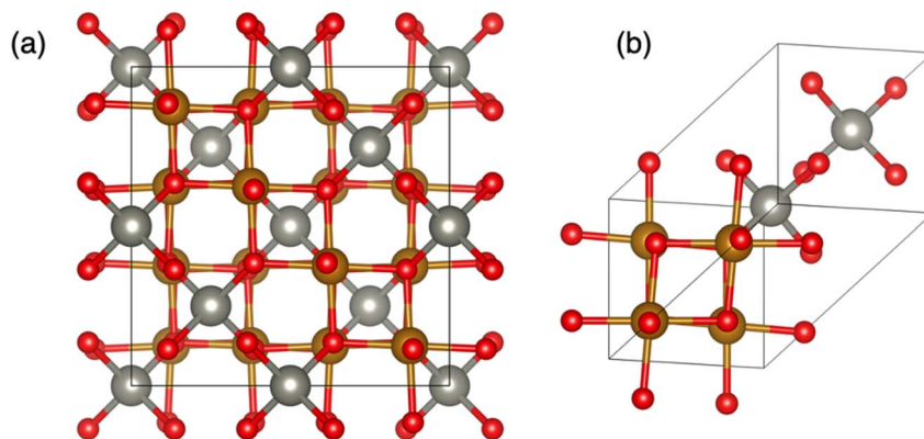
Fig. 1 Crystal structure of M\text{Fe}_2\text{O}_4 spinels represented by (a) the conventional cubic cell and (b) the primitive unit cell. Colour scheme: tetrahedral (Td) sites = silver; octahedral (Oh) sites = gold; oxygen = red.
