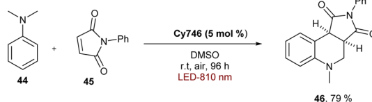
b) \alpha -nitrogen radical
