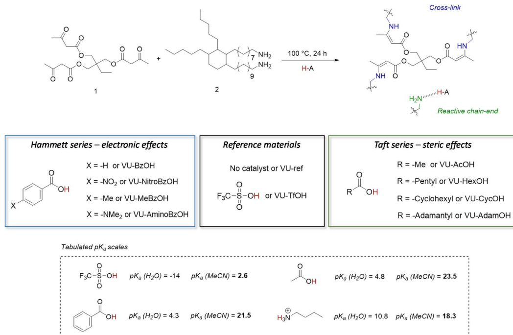
Fig. 2 Design of vinylogous urethane based vitrimers with thermoswitchable catalysis of bond exchange. The aim is to control the tendency of protonation or hydrogen bonding by changing the electronic and/or steric environment of the carboxylic acid additive, which results in a change in formal pK_a values. 67
