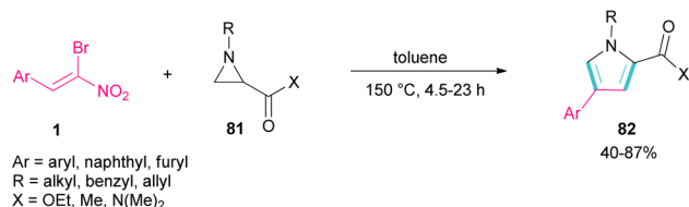
Scheme 34 Cataly-free reaction of unactivated aziridines with \beta -bromo- \beta -nitrostyrenes.
