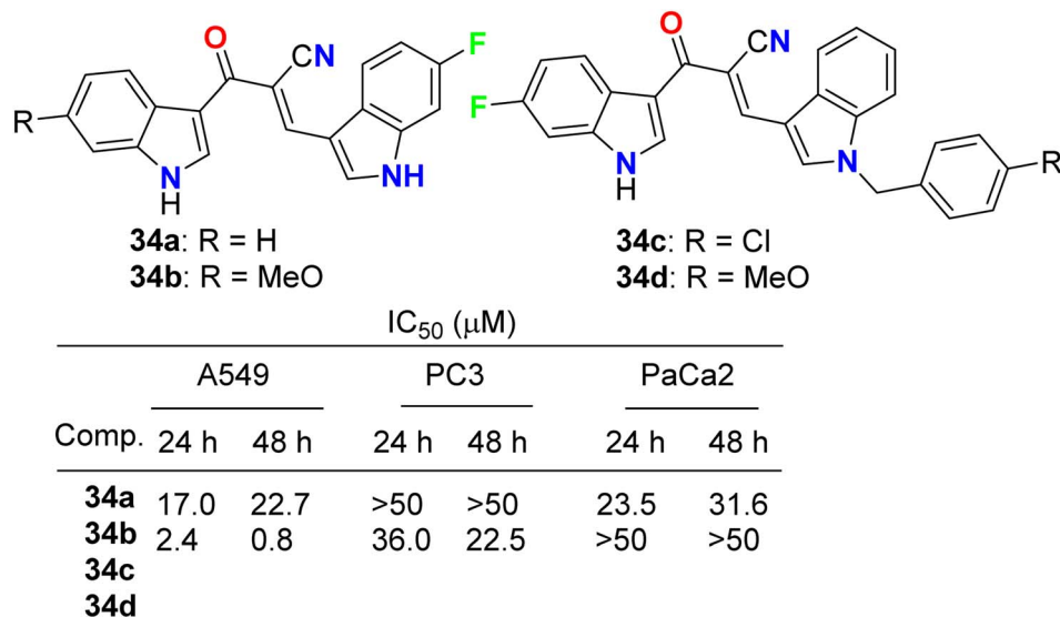
Fig. 21 Structure of fluorinated-indole derivatives 34a–d.
