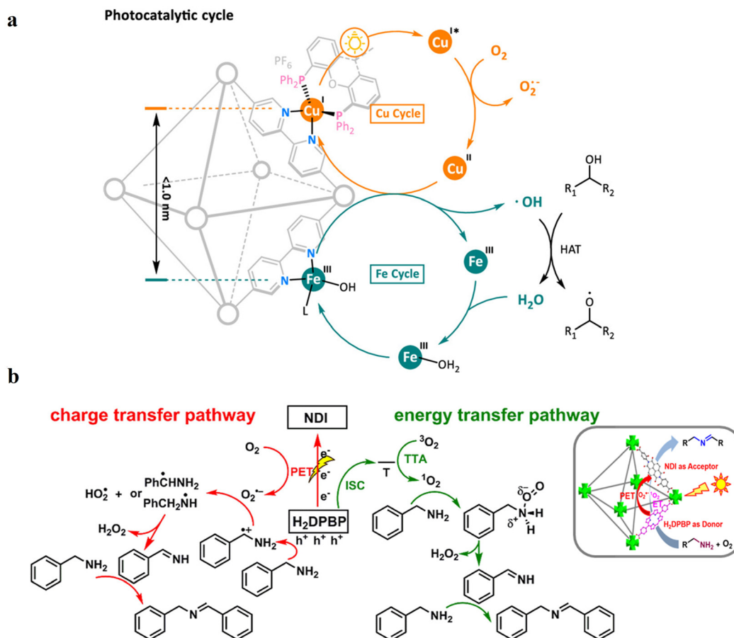
Fig. 16 (a) Proposed mechanism for the photocatalytic aerobic oxidation of alcohols to generate alkoxyl radicals with Zr 6 -Cu/Fe-1. Adapted with permission from ref. 184. Copyright 2021, the American Chemical Society. (b) Zr-NDI-H 2 DPBP as mixed-linker donor (H 2 DPBP) and acceptor (NDI)-based MOF model, and their photoinduced electron transfer (PET) process involved in photocatalytic oxidative coupling of amines. Adapted with permission from ref. 190. Copyright 2023, the American Chemical Society.
