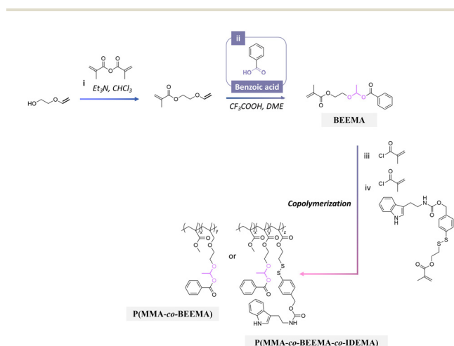
Fig. 25 Scheme of the synthesis of 2-(1-(benzoyloxy)-ethoxyl)ethyl methacrylate (BEEMA) and its copolymerization with either methyl methacrylate or 2-((4-(((2-(1 H -indol-3-yl)ethyl)carbamoyl)oxy)-methyl)phenyl)disulfanyl)ethylmethacrylate (IDEMA) and methyl methacrylate. 179
