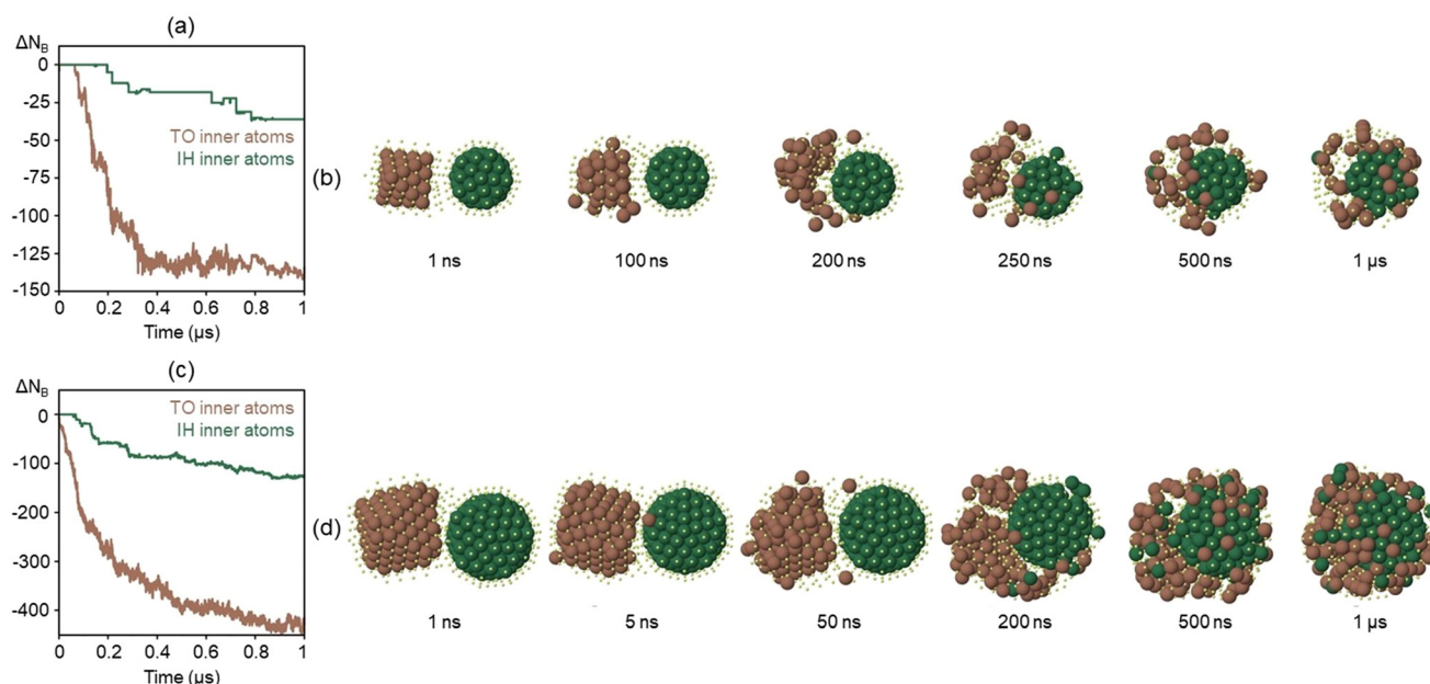
Fig. 9 Mobility of TO and IH inner atoms in two representative simulations ending up with the IH structural motif. (a and b) TO 140 ↔ IH 147 , AuPd composition, 650 K. (c and d) TO 314 ↔ IH 309 , AuPd composition, 750 K. Simulations are the same as in Fig. 4. (a and c) Evolution of \Delta N_B during the whole simulation. (b and d) Snapshots of the simulations, in which atoms are coloured according to their position before the collision: brown – atoms initially belonging to the inner part of the TO; green – atoms initially belonging to the inner part of the IH. All other atoms are displayed as small spheres.
