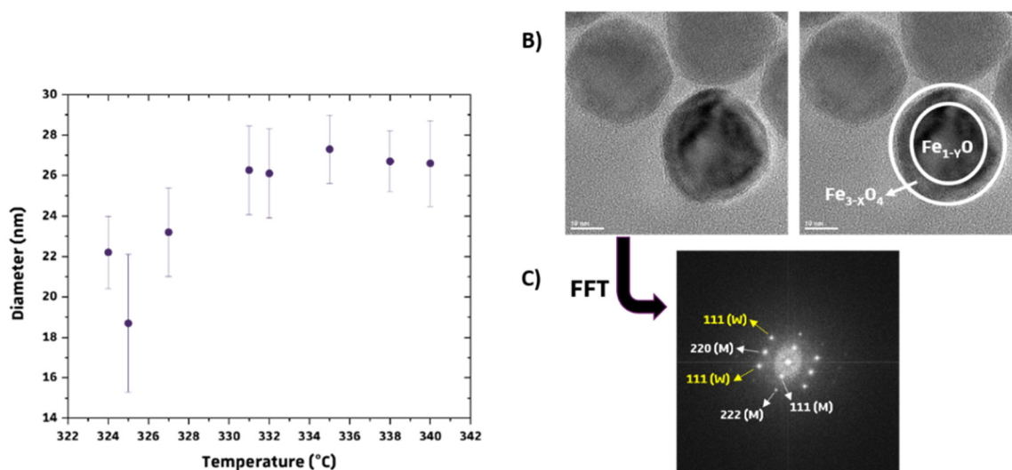
Fig. 2 (A) Mean diameter of IONPs synthesized using protocol P20_2 as a function of the reaction temperature, (B) HRTEM images of core-shell \text{Fe}_{1-x}\text{O}@\text{Fe}_3\text{O}_4 IONPs and (C) its corresponding FFT pattern with plane indication (W = wüstite plane, M = magnetite plane) (A).
