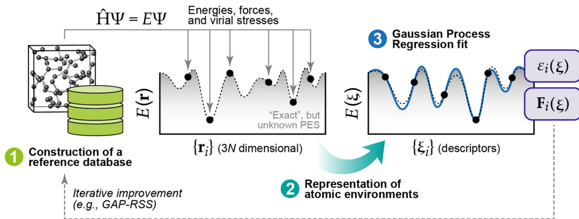
Fig. 4 Three main components required for GPs: (1) a robust reference database of quantum-mechanical data (usually generated with DFT), (2) a representation of the atomic environments associated with each reference point, and (3) the GPR model fit. This figure has been reproduced from ref. 69 with permission from the American Chemical Society, copyright 2021.
