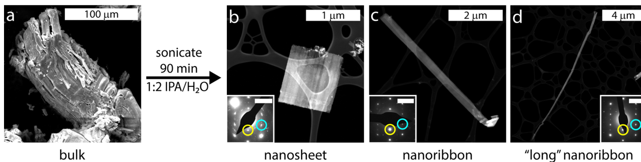
Fig. 2 When (a) bulk \text{KFeS}_2 is sonicated in 1 : 2 IPA/ \text{H}_2\text{O} for 90 min, it exfoliates into a mixture of (b) nanosheets and (c) nanoribbons, as well as occasional (d) particularly long nanoribbons. Although the morphologies are different, they all share the same crystal structure, as confirmed by the (b)–(d) insets) selected area electron diffraction patterns indexed to the [010] zone axis. The (002) diffraction spot is circled in cyan and the (200) is circled in yellow. The scale bar represents 5 \text{ nm}^{-1} . Note that the patterns have been rotated to the same direction for ease of comparison.
