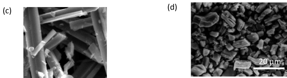
Figure 5. (a) Crystal structure of fibrous-like titanate (monoclinic) 72 ; (b) Crystal structure of lepidocrocite-like titanate (orthorhombic) viewed down along the a-axis 73 ; (c) FESEM image of fibrous-like titanate 73 ; (d) FESEM image of lepidocrocite-like titanate 74 . Panel (a) adapted with permission. 72 Copyright © 2010, American Chemical Society. Panel (b, c) adapted with permission. 73 Copyright © 1995, American Chemical Society. Panel (d) adapted with permission. 74 Copyright © 1998, American Chemical Society.
