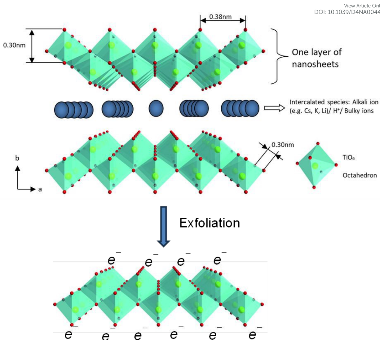
Figure 11. The polyhedral representation of crystal structure of layered lepidocrocite-like titania nanosheets viewed down along the c -axis and mono-layer titania nanosheets after exfoliation. Adapted from Ref. 88 with permission from the Royal Society of Chemistry.
