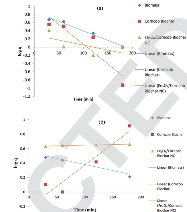
Fig. 15 Pseudo first order plot (a) Cr(IV) and (b) Ni(II).
