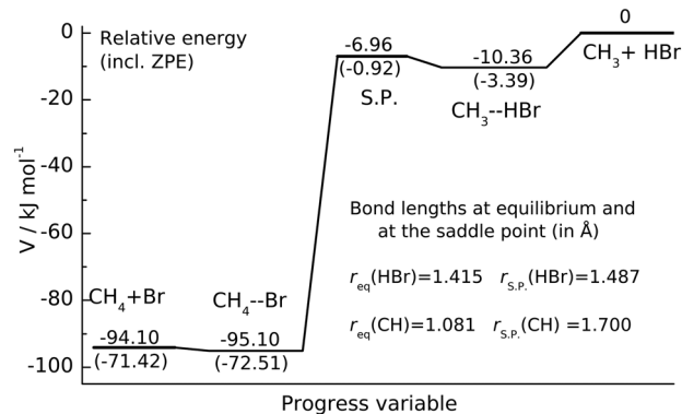
Fig. 1 Potential energy profile of CH 3 + HBr reaction. The energy levels of the stationary points characterizing the Czako–Góger–Szabó–Lendvai PES 15 are given in kJ mol -1 . The zero-point energy corrected energies are shown in parentheses. The S.P. denotes the saddle point.
