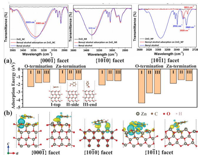
Figure 10. IR absorption of different ZnO nanomaterial before and after BnOH absorption. The range is focused on the O–H stretch. (a): Calculated absorption energy of benzyl alcohol in different facets on different facets of ZnO hexagons. (b): electron density prediction of varied facets of ZnO with adsorbed benzyl alcohol. Credit: H.
