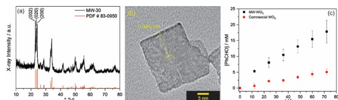
Figure 12. (Left) X-ray Diffraction data and (centre) TEM imaging of the obtained microwave synthesized \text{WO}_3 ; (right) Concentration of benzaldehyde, oxidation product of benzyl alcohol, over time during \text{WO}_3 photocatalysis. Black squares: microwave synthesized nanoplatelets; Red circles: commercial material. Credit: K. D. McDonald and B. M. Bartlett, RSC Adv. , 2019, 9, 28688-28694.
