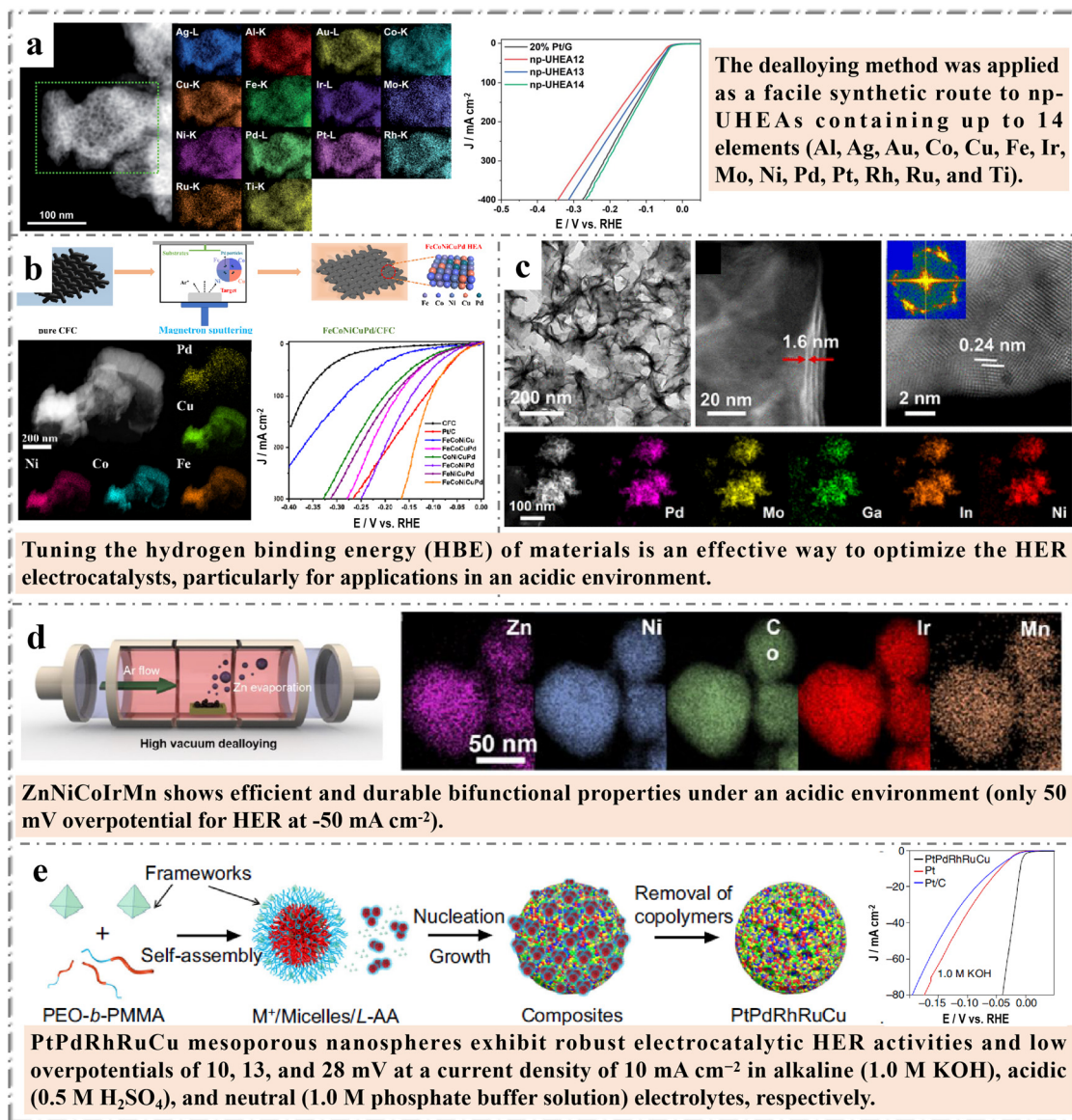
Fig. 5 Examples of HEMs in HER: (a) TEM image, EDX mappings and electrocatalytic performance of np-UHEAs (Al 87 Ag 1 Au 1 Co 1 Fe 1 Ir 1 Mo 1 -Ni 1 Pd 1 Pt 1 Rh 1 Ru 1 Ti 1 ). Reprinted with permission. 95 Copyright 2021, The Royal Society of Chemistry. (b) Fabrication schematic illustration, TEM image and corresponding EDX mappings and electrocatalytic performance of the FeCoNiCuPd film. Reprinted with permission. 96 Copyright 2022, Elsevier Ltd. (c) Electron microscopic characterization of high-entropy alloy PdMoGaInNi nanosheets. Reprinted with permission. 97 Copyright 2022, American Chemical Society. (d) Schematic illustration of selective Zn dealloying through vapor dealloying process and EDX mappings of ZnNiCoIrMn. Reprinted with permission. 98 Copyright 2023, Wiley-VCH; (e) Schematic illustration of PtPdRhRuCu mesoporous nanospheres and electrocatalytic performance of samples (polarization curves). Reprinted with permission. 99 Copyright 2023, Springer Nature.
