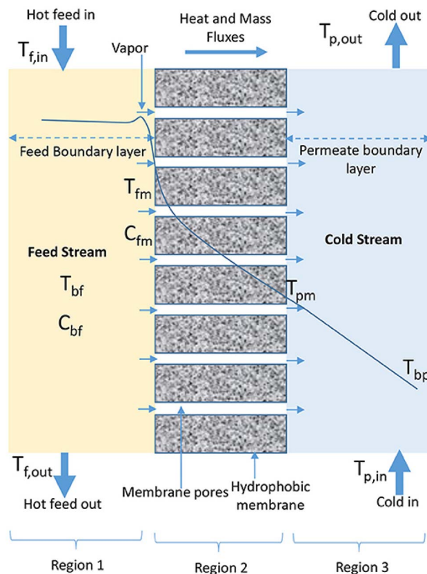
Fig. 4 Temperature polarization phenomenon in MD. T_{f,in} , T_{fm} , T_{pm} and T_{p,out} represent temperatures in the bulk feed solution, near the membrane surface (feed side), near the membrane surface (permeate side) and in the bulk permeate, respectively. 58
