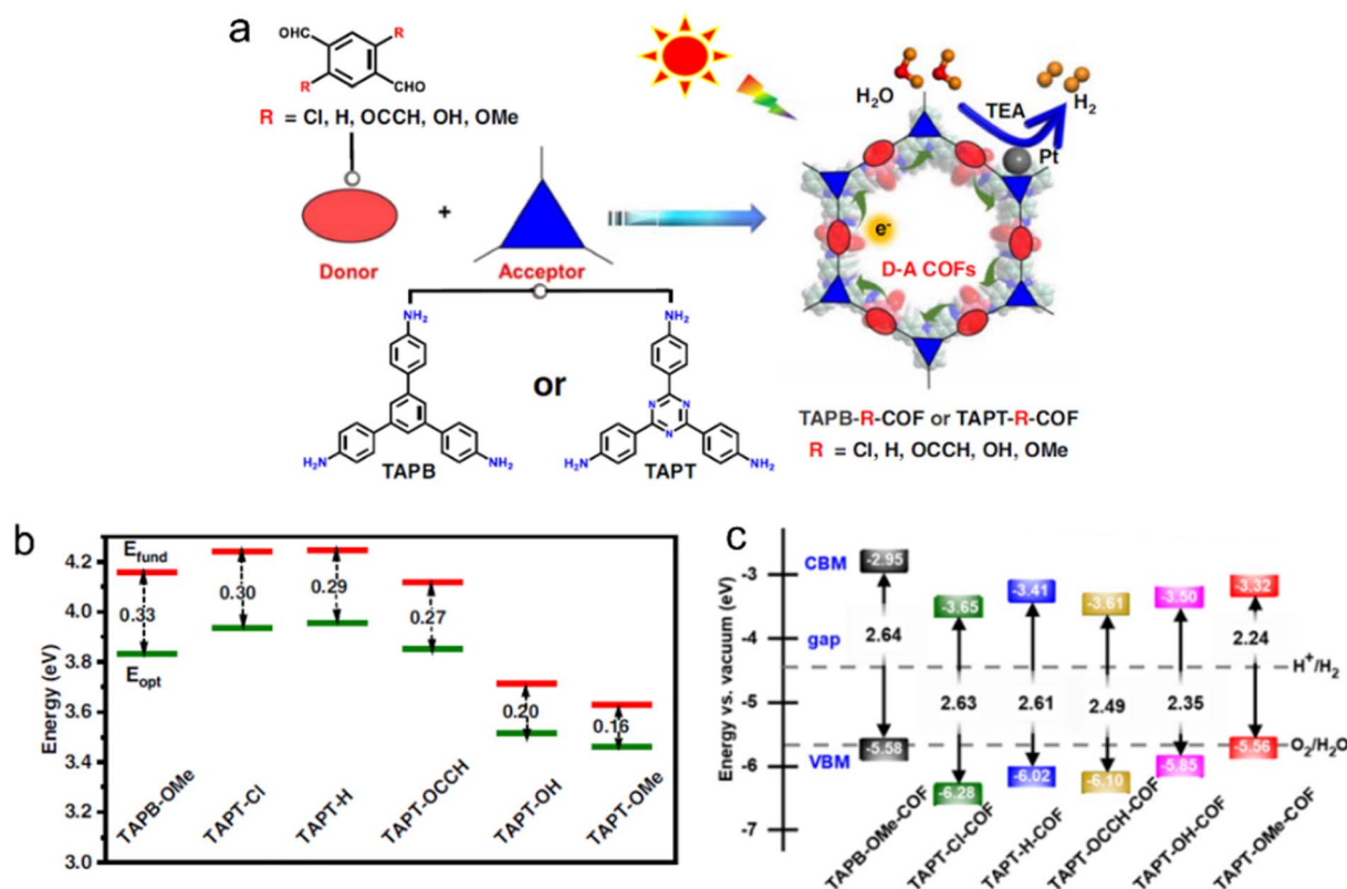
Fig. 10 (a) D–A COFs constructed from amine monomers and functionalized terephthalaldehydes for photocatalytic H 2 evolution under a 300 W Xe lamp ( \lambda > 380 \text{ nm} ) by using triethylamine as a sacrificial agent. TAPB, TAPT and TEA indicate 1,3,5-tris(4-aminophenyl)benzene, 1,3,5-tris(4-aminophenyl)triazine and triethylamine, respectively. (b) Extrapolation results of fundamental gap ( E_{\text{fund}} , red line) and optical gap ( E_{\text{opt}} , green line) energies of D–A pairs. E_b (exciton binding energy) = E_{\text{fund}} - E_{\text{opt}} . (c) The calculated bandgap and band position of COFs relative to the vacuum level. The dashed lines are the redox potential of water at pH = 0. Reproduced with permission from ref. 100 . Copyright 2023, Springer Nature.
