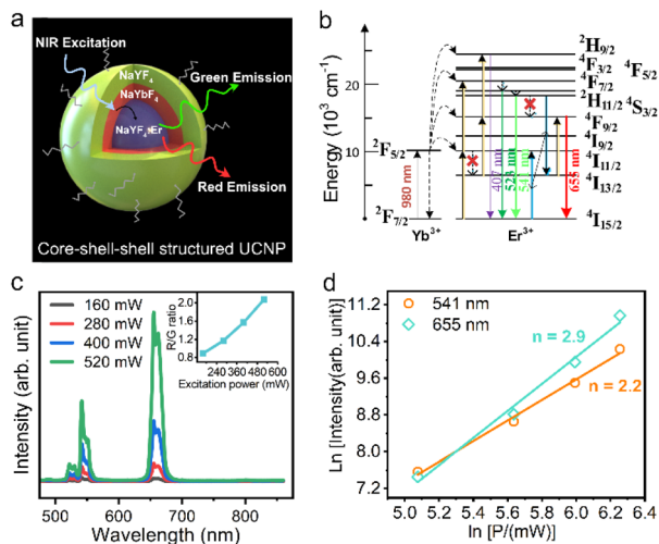
Fig. 3 (a) Schematic diagram showing the emission properties of UCNP, (b) schematic illustration of the proposed energy transfer mechanism, (c) power-dependent emission spectra and (d) the relationship between emission intensity and excitation power of core-shell-shell structured \text{NaYF}_4\text{:}10\%\text{Er@NaYbF}_4\text{:}10\%\text{Er@NaYF}_4 UCNP.
