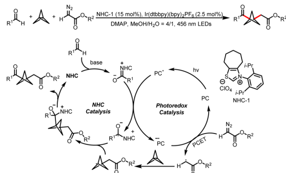
Scheme 9 Synthesis of 1,3-disubstituted bicyclo[1.1.1]pentane ketones.
