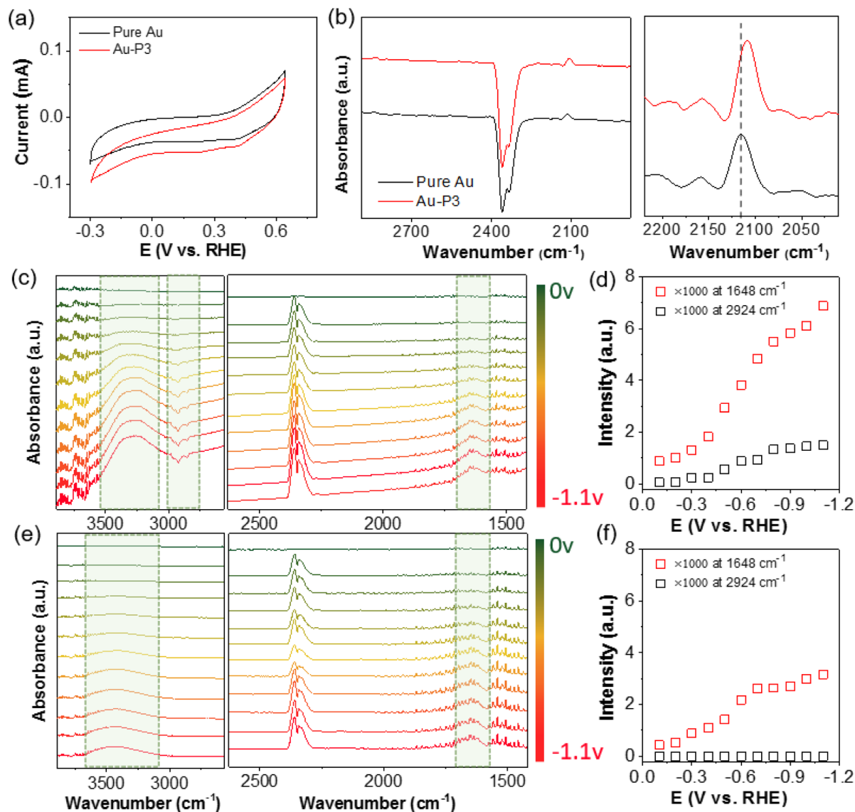
Fig. 4 Infrared spectroscopic study of Au electrodes with polymer NHC ligands. (a) CV scans in \text{N}_2 saturated 0.1 \text{ M KHCO}_3 and (b) in situ ATR-SEIRAS spectra obtained at -0.3 \text{ V}_{\text{RHE}} of AuNPs and Au-NHC-PS- b -PEO, respectively. In situ ATR-SEIRAS spectra and vibrational peak intensity study for Au-NHC-PS- b -PEO (c) and (d) and pure AuNPs (e) and (f) in \text{CO}_2 -purged 0.1 \text{ M KHCO}_3 under various reductive potentials. The spectra in (c) and (e) are background subtracted at 0 \text{ V} .
