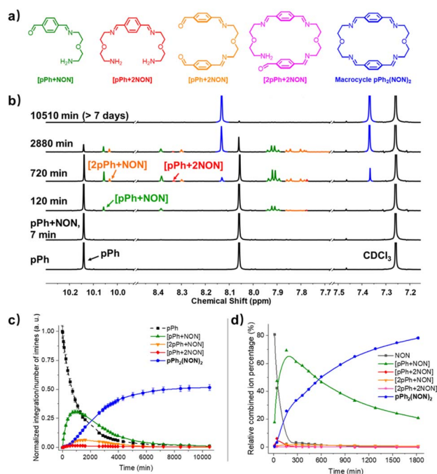
Fig. 2 (a) Chemical structures of the different intermediates and of \text{pPh}_2(\text{NON})_2 . (b) evolution of the 1 H NMR spectra (500 MHz, CDCl 3 , 23 °C) of a 1 : 1 mixture of \text{pPh} and NON ( [\text{pPh}]_0 = [\text{NON}]_0 = 3.6 \text{ mM} ) showing the formation of three intermediates and of the final macrocycle \text{pPh}_2(\text{NON})_2 after 7 min, 120 min, 720 min, 2880 min and 10 510 min. (c) 1 H NMR monitoring of the evolution of the species generated during \text{pPh}_2(\text{NON})_2 formation from a 1 : 1 mixture of \text{pPh} and NON as a function of time over 10 510 min. Error in 1 H-NMR signal integration: \pm 5\% . (d) HRMS-ESI monitoring of the species generated during the formation of the macrocycle \text{pPh}_2(\text{NON})_2 from a 1 : 1 mixture of \text{pPh} and NON ( [\text{pPh}]_0 = [\text{NON}]_0 = 2 \text{ mM} , 50/50 (v/v) CHCl 3 /MeOH, 25 °C) over 1820 min. The spectra and kinetic curves are coloured in accordance with the molecular structures. NB: the relative combined ion percentage is obtained by the ratio of combined ion count of each species to the sum of combined ion counts for all species at each time point. These data do not provide quantitative information about the relative amounts of each species identified by its mass, but, taken separately, they display the evolution of a given identified species during the course of the reaction. The curves are added to guide the eye.
