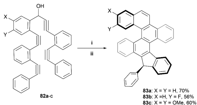
Scheme 16 Synthesis of nanographenes via alkyne-based “folding” technique; (i) 82 (1.0 equiv.), \text{Bu}_3\text{SnH} (1.4 equiv.), AIBN (0.3 equiv.), toluene 110\text{ }^\circ\text{C} , 14 h; (ii) Aq. HCl (2 M), rt, 3 h.
