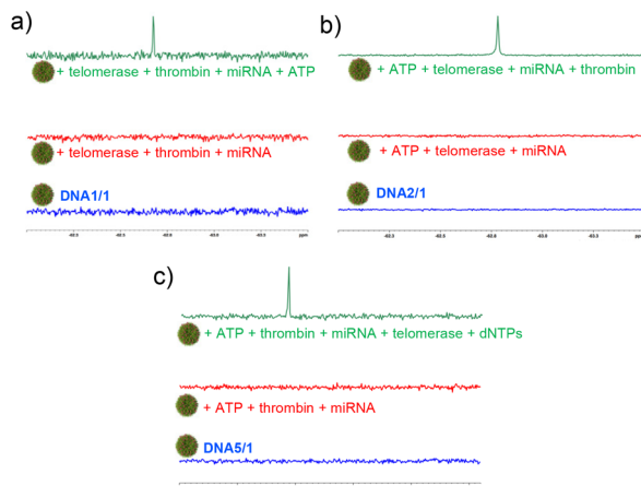
Fig. 4 19 F-NMR spectral responses of (a) DNA1/1 NPs towards ATP, (b) DNA2/1 NPs towards thrombin and (c) DNA5/1 NPs towards telomerase in the presence of a mixture of other nontargets.
