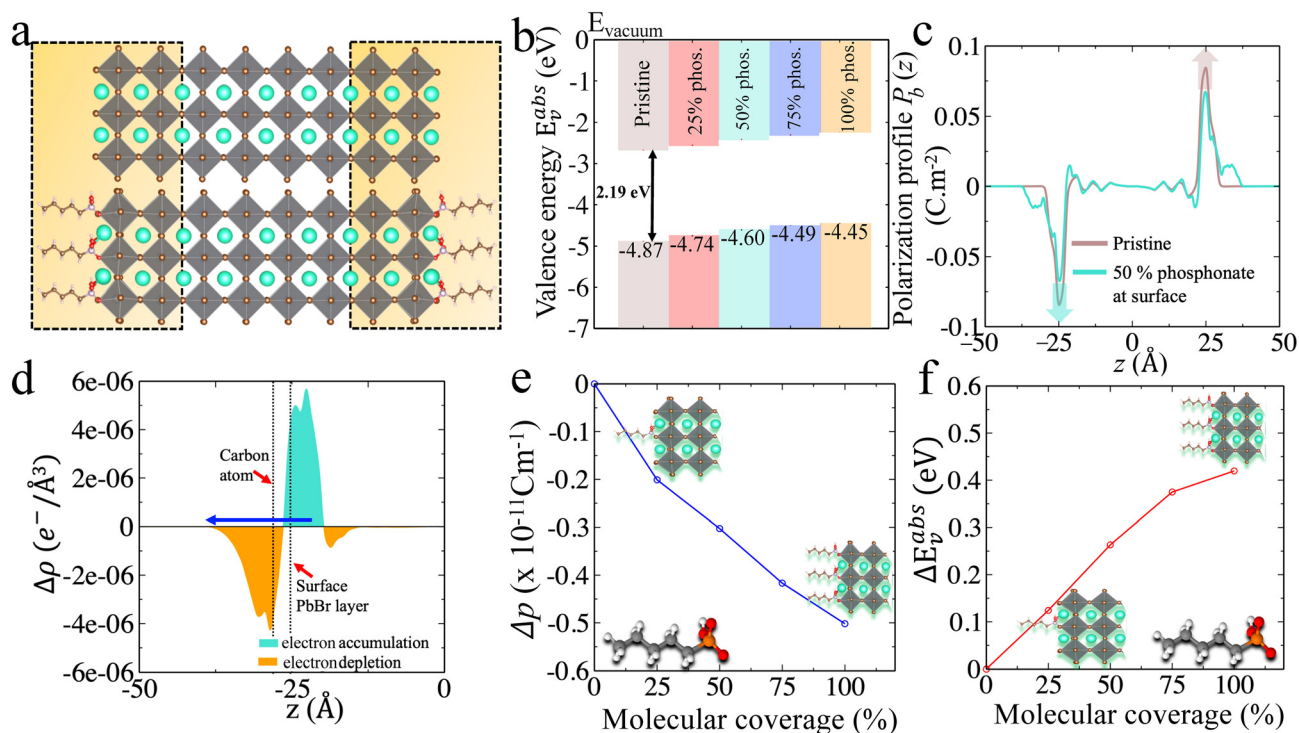
Fig. 2 (a) CsPbBr 3 CsBr terminated slabs without (top) and with (bottom) phosphonate ligands attached to the surface. The later is illustrated for 50% molecular coverage. (b) Valence energies for 0% to 100% surface coverage. (c) Polarization density profiles for 0% and 50% molecular coverage (for other concentrations see ESI, Fig. S7†). The integration of these polarization profiles result in the surface dipole densities (Table 2). (d) Variation of the electronic charge density upon functionalization with phosphonate for 50% molecular coverage. For clarity, only one side of the symmetric slab is shown. Orange and turquoise color represent electronic depletion and accumulation region, respectively, and the arrow indicates the net dipole direction. (e) Relation between the change in surface dipole density and the molecular coverage. (f) Relation between the change in the valence energies and the molecular coverage. The valence energy values are computed from the Hartree potential profiles.
