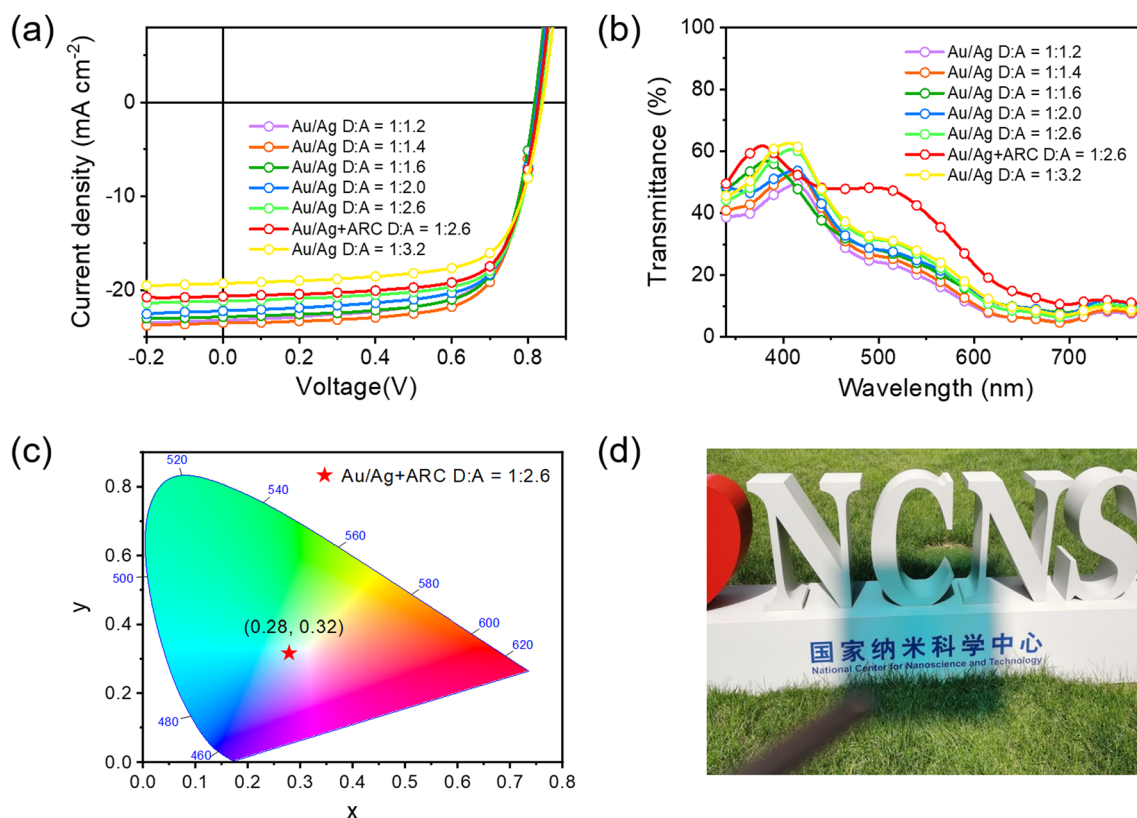
Fig. 5 (a) J - V curves of PBDTTTP:N3 semitransparent solar cells with different D/A ratios. (b) Transmittance spectra. (c) Coordinates of CIE 1931 for the best-LUE cell. (d) The photograph of a 1 \text{cm}^2 semitransparent cell made under optimal conditions.
