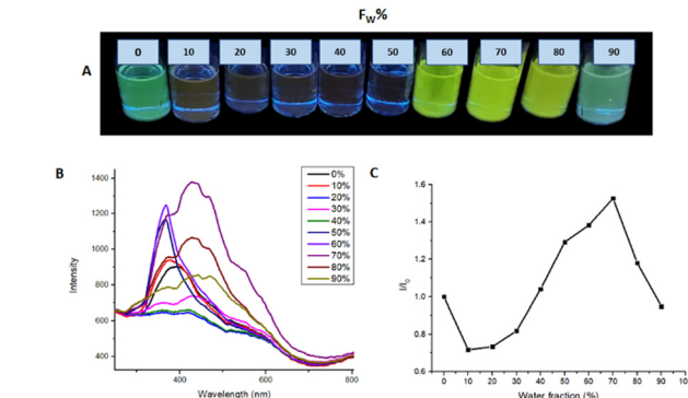
Fig. 7 (A) AIEE M2 samples under 366 nm to different THF/water ratios. (B) AIEE test emission spectrum. (C) plot of water fraction vs. I/I_0 .
