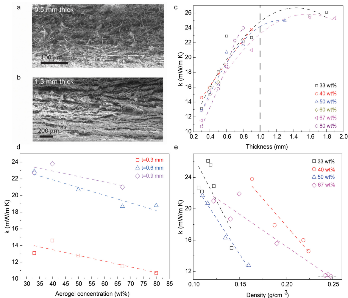
Fig. 2 (a) Cross-sectional SEM image of the membrane with a thickness of 500 μm. (b) Cross-sectional SEM image of the membrane with a thickness of 1.3 mm. (c) Thermal conductivity vs. thickness of the membrane with different concentrations. (d) Thermal conductivity vs. aerogel concentration for membranes with thicknesses of 0.3 mm, 0.6 mm and 0.9 mm. (e) Thermal conductivity vs. density for membranes with different aerogel concentrations.
