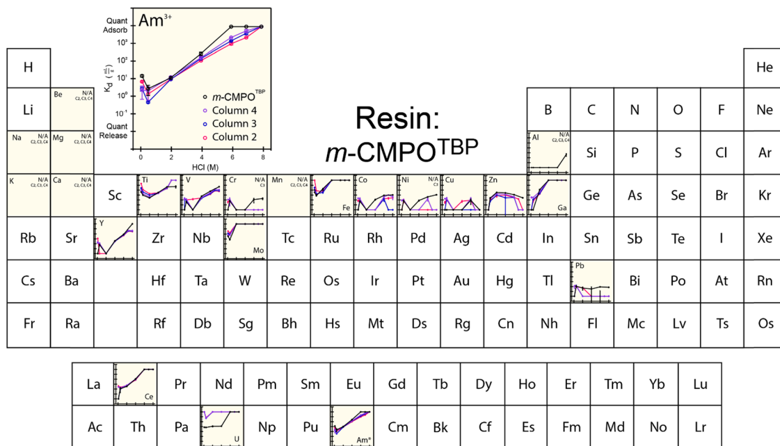
Fig. 3 Temperature controlled (25 °C) distribution coefficients ( K_d ) from 'veteran' m\text{-CMPO}^{\text{TBP}} resin for ^{241}\text{Am}_{(\text{aq})} (20 pCi) in HCl (0.1 to 8 M) with twenty-three metal contaminants present at 5 ppm. Measurements were made in triplicate and uncertainty is shown as the standard deviation of the mean (at 1\sigma ). Elements labeled with N/A were not adsorbed. The asterisk (*) indicates when analytes were present on a microscopic scale and used as a radiotracer.
