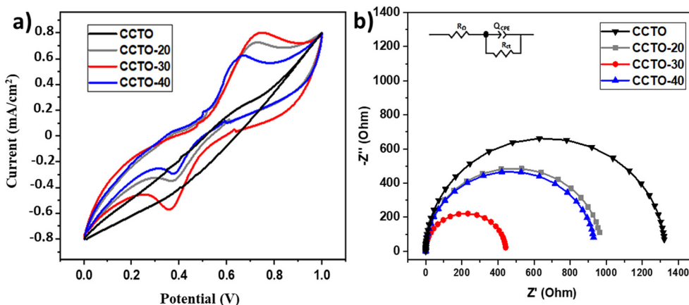
Fig. 6 (a) Cyclic voltammety curves obtained using CCTO, CCTO-20, CCTO-30 and CCTO-40 as electrodes in 1 M KOH (scan rate = 25 mV s -1 ). (b) Nyquist plots showing the electrochemical impedance spectroscopy data for CCTO, CCTO-20, CCTO-30 and CCTO-40.
