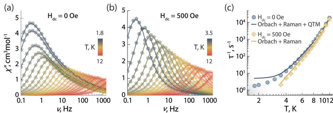
Fig. 2 Frequency dependence of the out-of-phase ( \chi'' ) magnetic susceptibility as a function of temperature obtained in absence of an external dc magnetic field (a) and under an applied static field of 500 Oe (b). (c) Temperature dependence of the magnetic relaxation times ( \tau ) in absence (blue circles) and in the presence of a 500 Oe applied field (yellow diamonds). Solid lines in (c) are the best fit to the experimental data using eqn (1).
